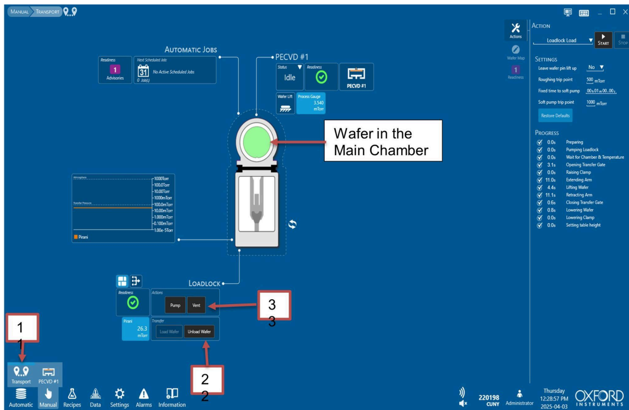
Image 6, Unloading steps for wafer/chips after Condition/Deposition processes
