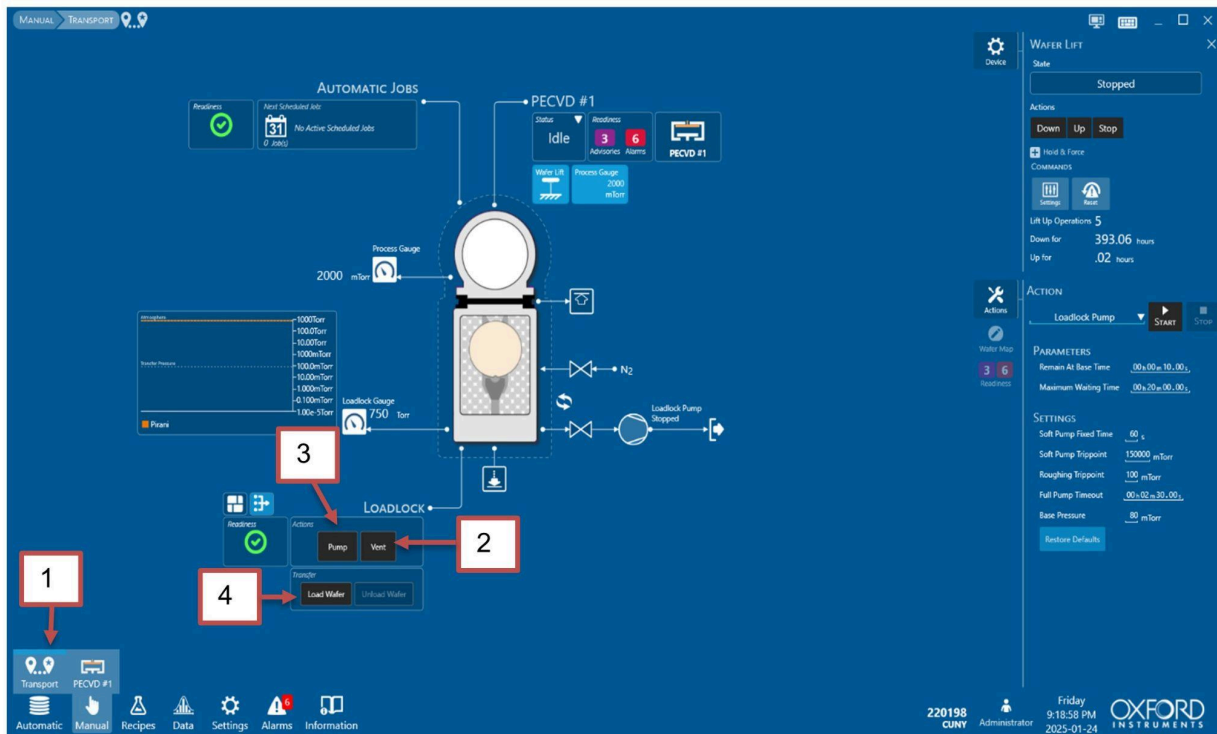
Image 4, Loading steps for wafer/chips for Condition/Deposition/Clean processes
