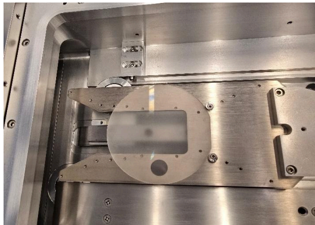
Image 11 Flat Edge of the Sapphire Cleaning Wafer on the load arm
