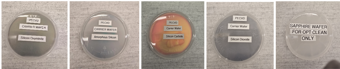
Image 10: 4" Wafers that use the PECVD conditioning or carrier wafer to support small chips. SiON, A-Si, SiO 2 and Sapphire wafers.
