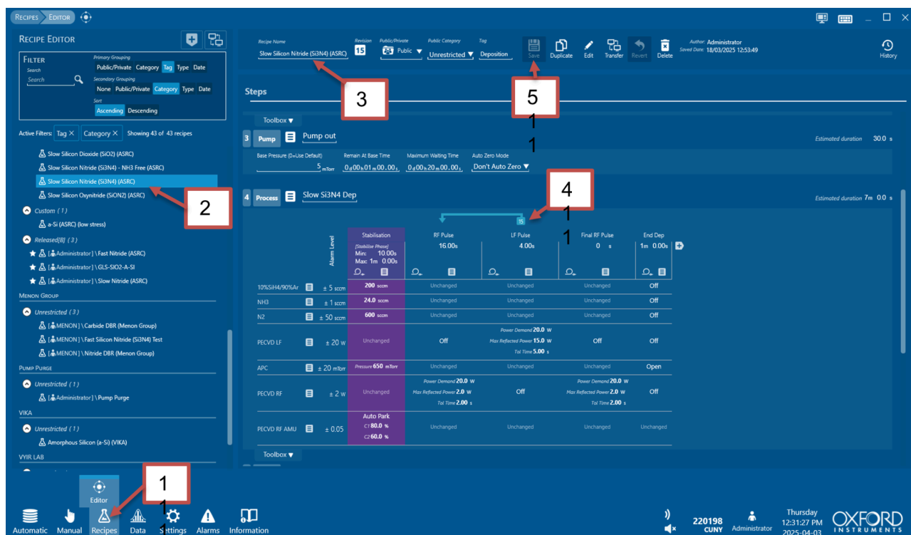
Image 8, Changing deposition time on the Nitrite Recipe or recipe that has the deposition process with a number of cycles.
