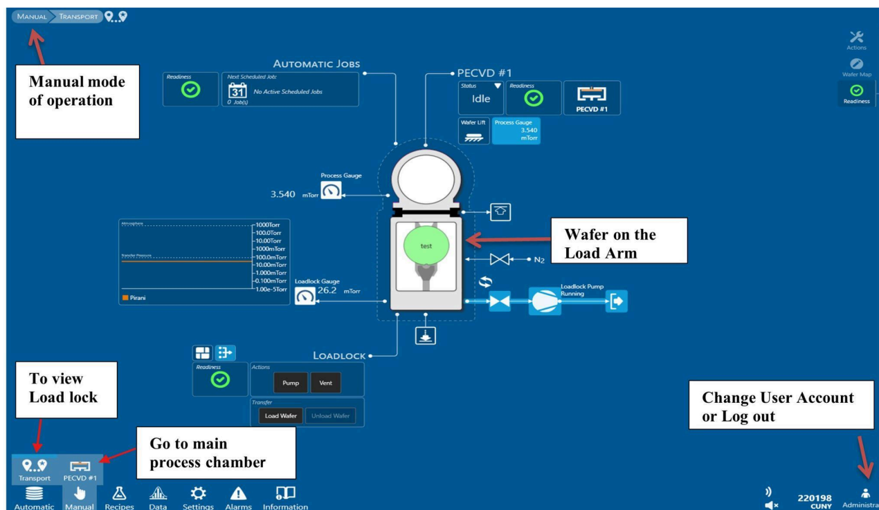
Image 2, general cartoon view of PTIQ screen
